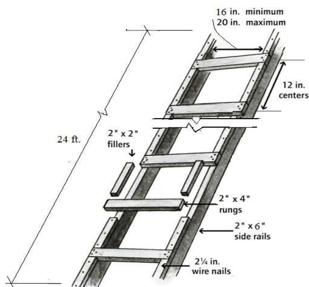
Figure 1: Single-Cleat Ladder
